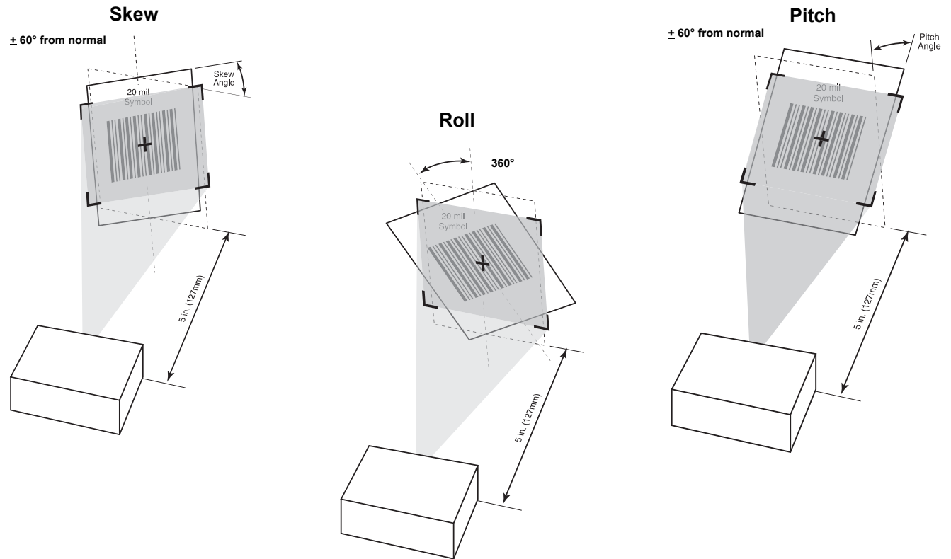
Figure 9 Skew, Pitch and Roll
