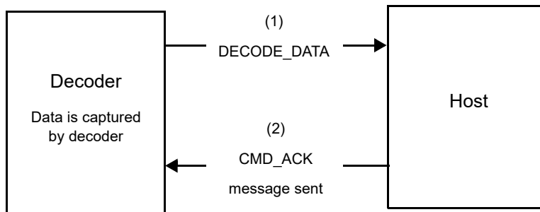
Figure 10 ACK/NAK Enabled and Packeted Data
