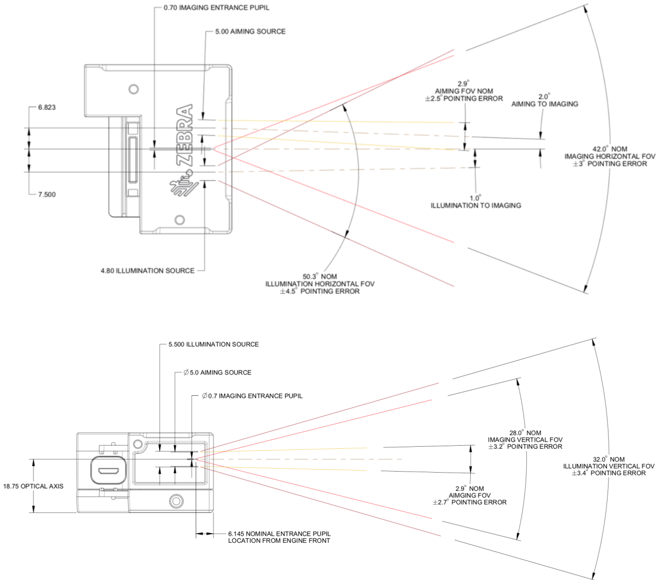
Figure 6 MS4717 Optical Path and Exit Window
