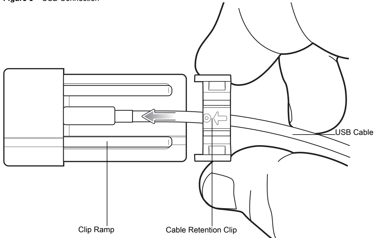
Figure 5 USB Connection
